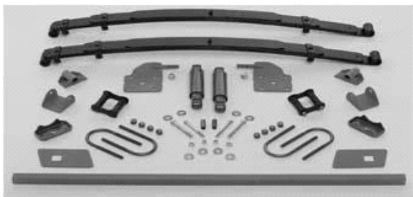
06-1809 - PARALLEL LEAF REAR SUSPENSION KIT DIRECT FIT AVAILABLE FOR SEVERAL MODELS UNIVERSAL KIT ALSO AVAILABLE. SPECIFY YEAR, MAKE AND MODEL WHEN ORDERING
