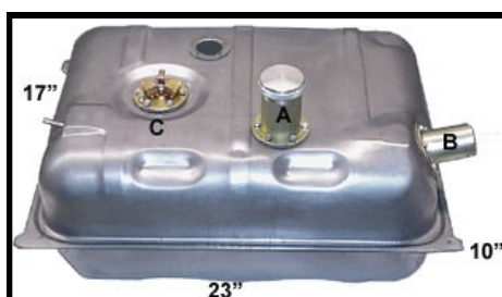
Universal Car or Truck Tank
