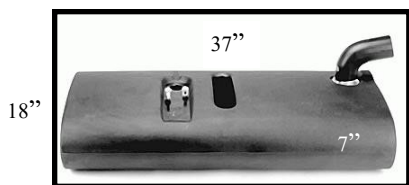
1935-36 Dodge/Plymouth Car Gas Tank
