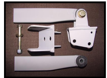
Chrysler 20-1263 V-10 Viper (1992-2002)
