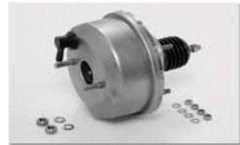
7" SINGLE DIAPHRAM BOOSTER 05-1512 - PLAIN 05-1512C - CHROME
