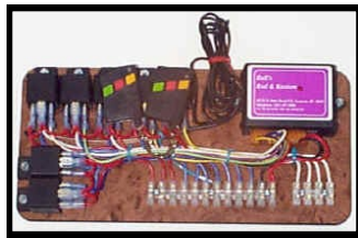
Pre-Built RPM 3:7 Remote Module
