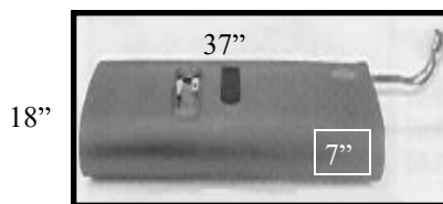
1937-39 Dodge/Plymouth Car Gas Tank
