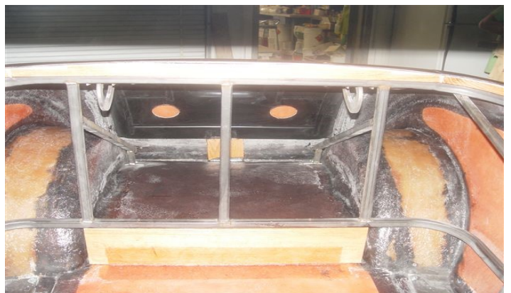
1934 Plymouth Roadster Fiberglass Body (See Descriptions and Pricing on Page 81-82)
